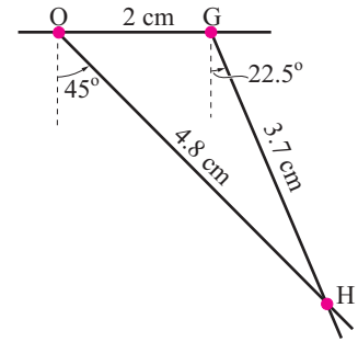
Figure 1.68: Method III: Find point H as the intersection of two known lines.
