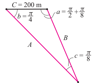
Figure 1.69: Solving “A walk” using the law of sines.
