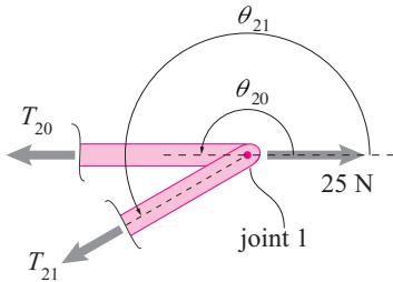
Figure 6.45: Free-body diagram of joint 1 on the truss of fig. 6.41 on page 2.
