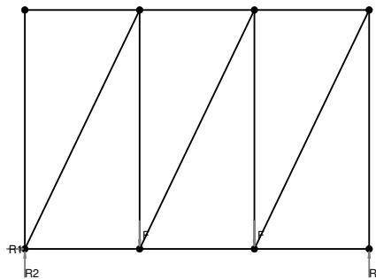
Figure 1: Truss system 1
