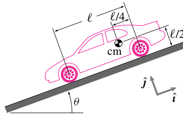
Problem 14.31: A car skidding downhill on a slope of angle \theta
