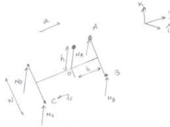
Problem 14.48: Given normal force at D, skidding at C.
