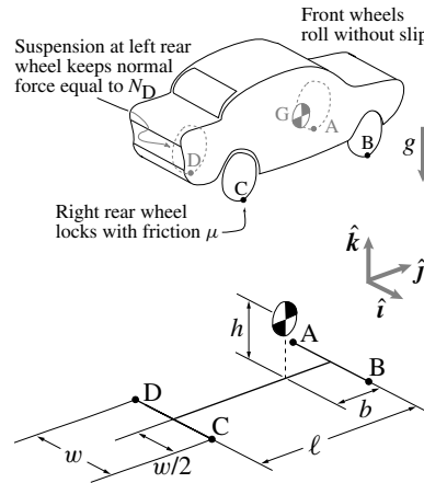
Problem 14.48: Given normal force at D, skidding at C.
