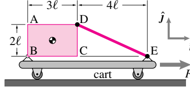
Problem 14.2.11: Uniform plate supported by a hinge and a cable on an accelerating cart.
