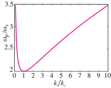
Figure 11.8: The ratio \omega_p/\omega_s of the two natural frequencies as a function of the spring stiffness ratio k_1/k_2 .
