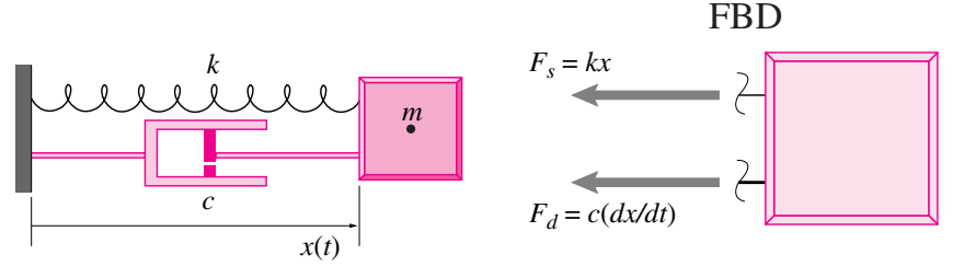
Figure 11.3: A mass spring dashpot system, or damped harmonic oscillator. The free-body diagram of the mass shows the tension in the dashpot.
