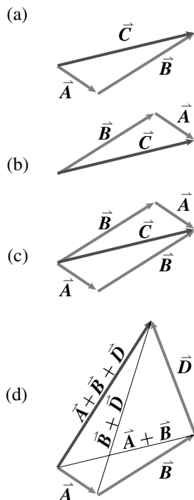
Figure 2.3: (a) tip to tail addition of \vec{A} + \vec{B} , (b) tip to tail addition of \vec{B} + \vec{A} , (c) the parallelogram interpretation of vector addition which shows the commutative law of vector addition: \vec{A} + \vec{B} = \vec{B} + \vec{A} , and (d) The associative law of vector addition: (\vec{A} + \vec{B}) + \vec{D} = \vec{A} + (\vec{B} + \vec{D}) .
