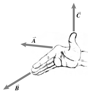
Figure 2.27: The right hand rule for determining the direction of the cross product of two vectors. \vec{C} = \vec{A} \times \vec{B} .
