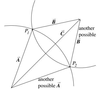
Figure 2.48: Solving a vector triangle where vectors \vec{A} and \vec{B} have known magnitude but unknown direction.
