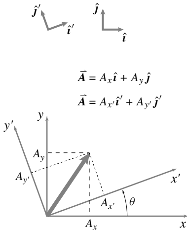
Figure 2.19: The dot product helps find components in terms of tilted unit vectors. For example, A_{y'} = \vec{A} \cdot \hat{j}' = A_x(\hat{i} \cdot \hat{j}') + A_y(\hat{j} \cdot \hat{j}') = A_x(-\sin \theta) + A_y(\cos \theta) .
