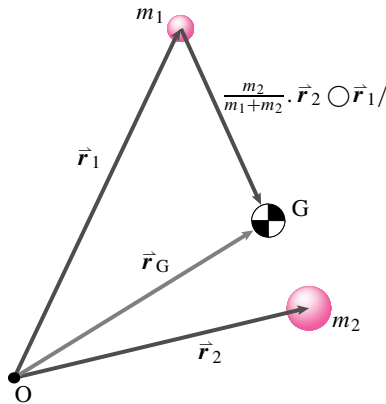
Figure 2.69: Center of mass of a system consisting of two points.
