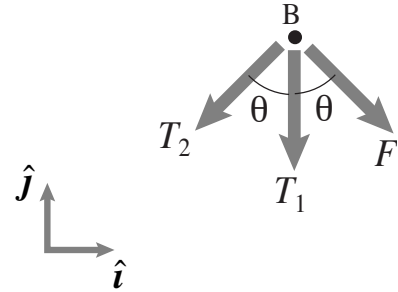
Figure 4.9: The free body diagram of the pin at B. Although we can see that rod AB is in compression, we use tension as positive and let the solution take care of the proper sign.
