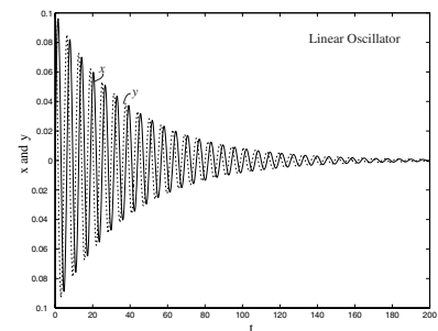
Figure 9.12: Numerical solution of the linear ODE \ddot{x} + c\dot{x}^2 + kx = 0 with initial conditions x(0) = 0 and \dot{x}(0) = 0.1 .
