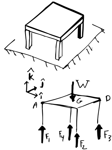
Figure 4.71: A symmetric 4 leg table on a flat floor. Statics is insufficient to find the 4 forces of the ground on the table. The full weight could be carried by either diagonal pair of legs.
