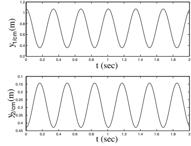
Figure 9.56: Numerically obtained solutions y_{1/cm}(t) and y_{2/cm}(t) .
