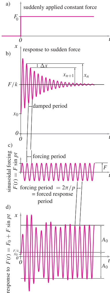
Figure 9.81: Transient response. (a) shows a suddenly applied force F_0 . The response (b) to this force is a motion that starts at the initial position x_0 ( x_0 > 0 in this illustration) and then oscillates about the new equilibrium F_0/k . The motion is identical to unforced motion, but offset. Thus it can be used to evaluate the rate of decay of oscillation and the damped period of oscillation. (c) A sinusoidal forcing causes. (d) the response if the mass is released at x = x_0 and suddenly both a constant force F and a sinusoidal force F \sin pt are applied. The motion eventually settles into a sinusoidal oscillation at the forcing frequency (which is a little longer period than the damped oscillation in this illustration) with amplitude A_0 .
