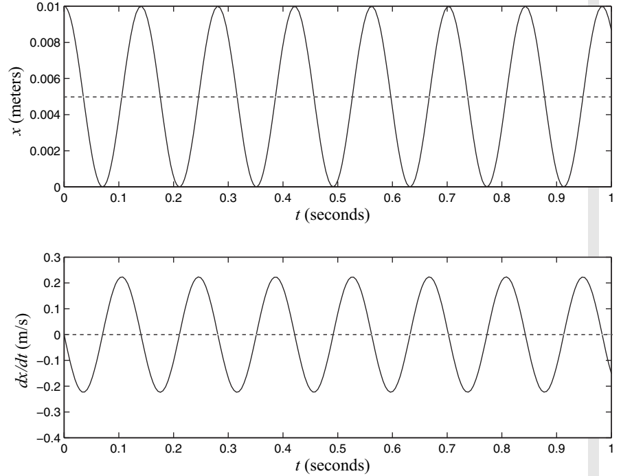
Figure 9.85: Displacement of the mass as a function of time. Note that the mass oscillates about a nonzero value of x .
