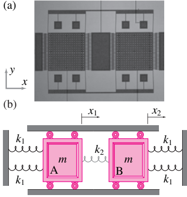
Figure 9.61: A MEMS vibratory gyroscope: (a) a micrograph of the two-mass structure. Each inertial mass (the plates with holes) is approximately 1 \text{ mm} \times 1 \text{ mm} \times 15 \mu\text{m} . The beams that hang the two masses act as springs. The comb drives on the left and right side of the two masses are used to drive the two masses to oscillate in the x -direction at their resonant frequencies. (b) a two degree of freedom spring-mass model of the driven gyroscope structure (without any damping).
