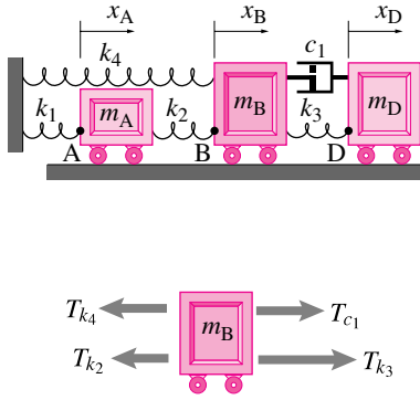
Figure 9.47: A system with 3 masses, 4 springs and a dashpot. Also shown is free body diagram of mass B.
