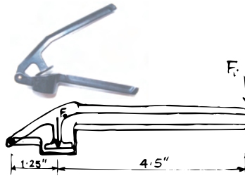
Filename:pfig6-lever-garlicpress
