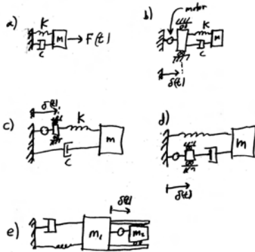
Figure 9.77: In all cases shown above the same forced oscillator eqn. (9.75) applies. In (a) a literal force is applied. In all the other cases the “forcing” is by a motor that moves something back and forth a distance \delta . In (b) the support moves. In (c) and (d) just the spring or just the dashpot end is displaced. In (e) an extra mass is moved relative to the main mass.
