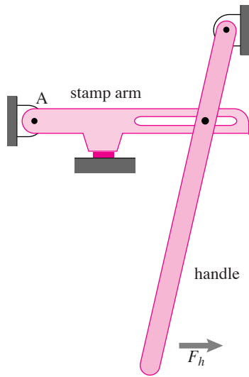
Figure 6.50: An improved stamp machine.
