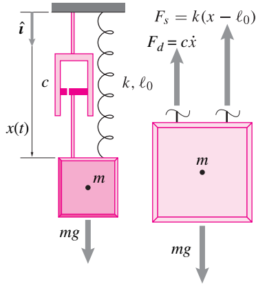
Figure 9.78: A mass hangs from a spring and dashpot. Its distance x from the support is due to the rest length \ell_0 of the spring, and the stretch of the spring.
