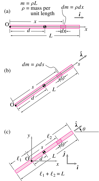
Figure 2.70: Where is the center-of-mass of a uniform rod? In the middle, as you can find calculating a few ways or by symmetry.
