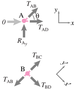
Figure 5.14: Free-body diagrams of joints A and B. From the given geometry, \theta = \pi/4 .
