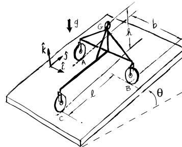
Filename:pfigure-threewheelparked
