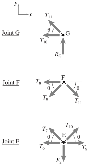
Figure 5.19: Free-body diagrams of joints G, F, and E. From the given geometry, \theta = 45^\circ .
