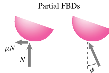
Figure 3.28: Two ways of characterizing friction: the friction coefficient \mu and friction angle \phi .
