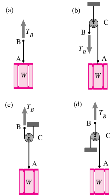
Figure 6.35: a) Lifting a weight, b) a pulley lets you pull down instead of up, c) a pulley halves the needed pull, d) a pulley doubles the needed pull.
