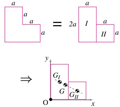
Figure 2.73: The center-of-mass of the ‘L’ shaped object can be found by thinking of it as a rectangle plus a square.
