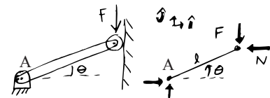
Figure 6.30: A simple toggle mechanism. Moment balance about point A gives that N = F/\tan \theta so if \theta is small N is large.
