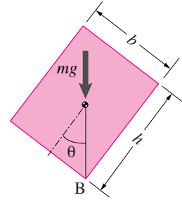
Figure 4.53: The impending tipping condition \tan \theta = \gamma \equiv b/h , provided \tan \theta \leq \mu .
