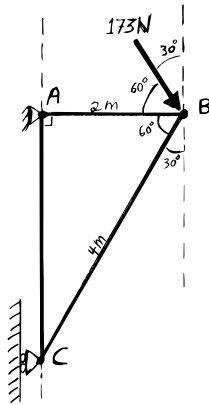
Filename:S03q3a-truss
