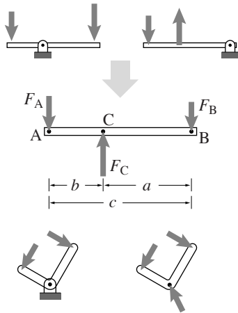
Figure 6.26: A lever can have the pivot in various places. The free body diagram looks the same in any case.
