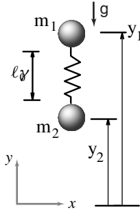
Figure 9.53: Filename:fig5-6-hopper
