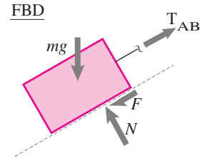
Figure 4.40: Pulling a block up a frictional slope with related FBD. As in the previous example, the pair N and F represent the net normal and frictional force.
