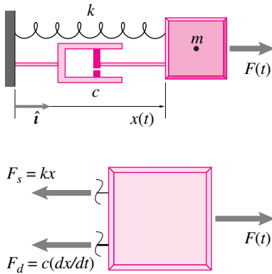
Figure 9.76: A forced mass-spring-dashpot is just a mass held in place by a spring and dashpot but pushed by a force F(t) from some external source.
