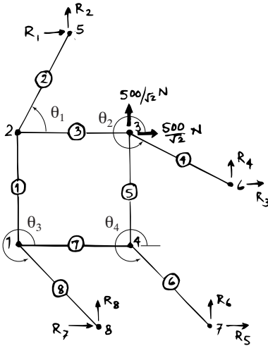
Figure 5.43: Free-body diagram of the truss along with bar and joint numbers. From the given geometry, \theta_1 = \pi/3 , \theta_2 = 11\pi/6 = -\pi/6 , and \theta_3 = \theta_4 = \pi/4 . Assuming the bar length to be \ell , we can write the coordinates of all joints in terms of \ell and \theta 's. For example, x_5 = \ell \cos \theta_1 , y_5 = \ell + \ell \sin \theta_1 .
