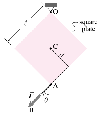
Figure 2.38: The moment of force F about point C is Fd and acts clockwise.
