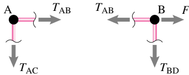
Figure 5.65: Free body diagrams of joints A and B from 5.64b. The solutions to the equilibrium equations are in conflict. That the equilibrium equations can't be satisfied means the structure cannot carry the given load. It is not rigid.
