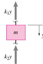
Figure 9.36: Free body diagram of the mass.
