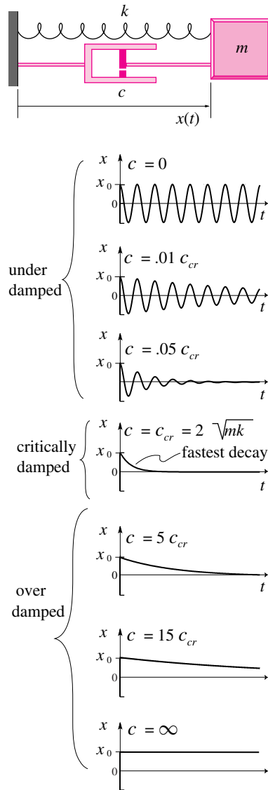
Figure 9.30: The effect of varying the damping with a fixed mass and spring. In all the plots the mass is released from rest at x = x_0 . In the case of underdamping, oscillations persist for a long time, forever if there is no damping. In the case of over-damping, the dashpot doesn't relax for a long time; it stays locked up forever in the limit of c \rightarrow \infty . The fastest relaxation occurs for critical damping.
