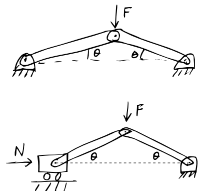
Figure 6.31: Two bars in a toggle mechanism.
