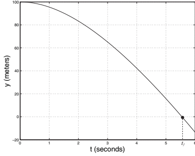
Figure 9.18: A graph of y(t) = h - \frac{mg}{c} \left( \frac{m}{c} e^{-\frac{c}{m}t} + t - \frac{m}{c} \right) for determining t_f when y = 0 . This is the same as solving eqn. (9.19) for t_f .
