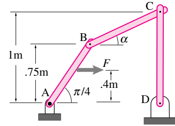
Figure 3.21: A four bar linkage.
