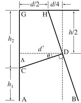
Figure 5.54: The geometry of h_1 and h_2 . Since d' = 3d/4 , \Delta = d' \tan \theta and \tan \theta = \frac{d/2}{h} , we get \Delta = \frac{3d}{4} \frac{d}{2h} = \frac{3d^2}{8h} and h_1 = h/2 - \Delta , h_2 = h/2 + \Delta .
