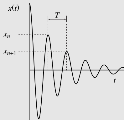
The logarithmic decrement method. D = \ln(x_n/x_{n+1})
