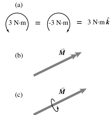
Figure 2.31: Optional drawing methods for moment vectors. (a) shows an arced arrow to represent vectors having to do with rotation in 2 dimensions. Such vectors point directly out of, or into, the page so are indicated with an arc in the direction of the rotation. (b) shows a double-headed arrow for torque or rotation quantity in three dimensions. (c) is another notation for a 3D vector quantity that uses rotations. But a vector is a vector and no special notation is usually used for vectors that concern turning or rotation.
