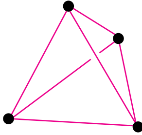
Figure 5.63: A tetrahedron is the simplest rigid truss in 3D that does not depend on grounding.
