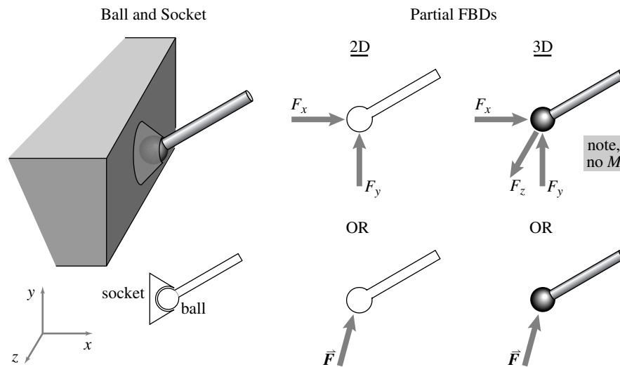
Figure 3.9: A ball-and-socket joint allows all relative rotations and no relative translations so reaction forces, but not moments, are shown on the partial free-body diagrams. In two dimensions a ball-and-socket joint is just like a pin joint. The top partial free-body diagrams show the reaction in component form. The bottom illustrations show the reaction in vector form.
