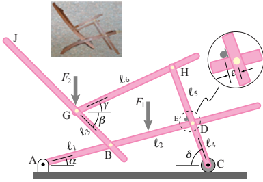
Figure 5.55: Dimensions: \ell_1 = 45 cm, \ell_2 = 60 cm, \ell_3 = 30 cm, \ell_4 = 30 cm, \ell_5 = 70 cm, \epsilon = 2.5 cm, \alpha = 15^\circ , \beta = 45^\circ , \gamma = 25^\circ , and \delta = 70^\circ . Loads: F_1 = 500 N and F_2 = 200 N
