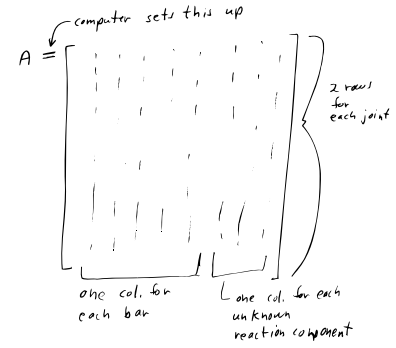
Figure 5.38: The matrix [A] contains all the coefficients in the linear joint equations. It is made of sines and cosines of bar angles and the direction cosines of reaction-force directions.
