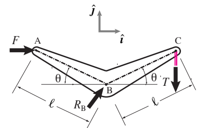
Figure 4.38: Free body diagram of the structure with rod CD cut just below C.
