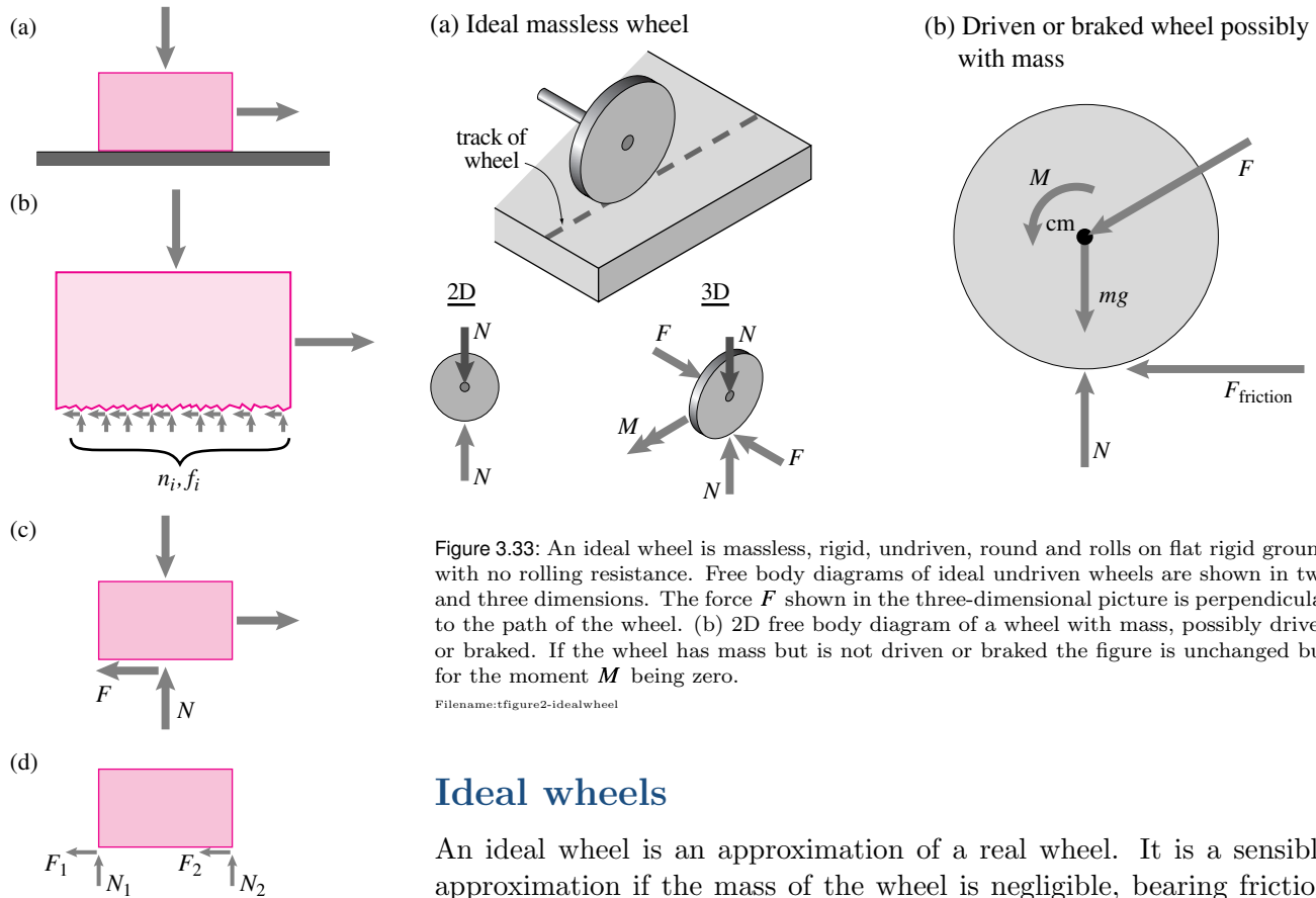
Figure 3.34: The contact forces of a block on a plane can be sensibly modeled in various ways.
