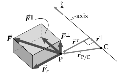
Figure 2.25: Moment about an axis
