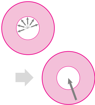
Figure 2.54: Frictionless wheel bearing. All the bearing forces are equivalent to a single force acting at the center of the wheel.
