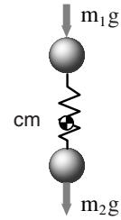
Figure 9.57: Free body diagram of the hopper as a single system. The spring force does not show up here since it becomes an internal force to the system
