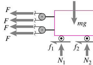
Figure 3.40: Free-body diagram of the cart.
