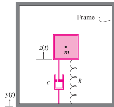
A single degree of freedom spring-mass model of an accelerometer.
