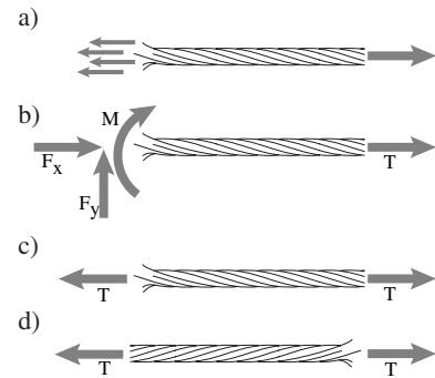
Figure 4.60: a) free body diagram of the right part of the rope, b) the same free body diagram, with the force distribution at the cut replaced with an equivalent force couple system, c) further simplified by using the laws of mechanics, and d) a free body diagram of the left portion of the rope.
