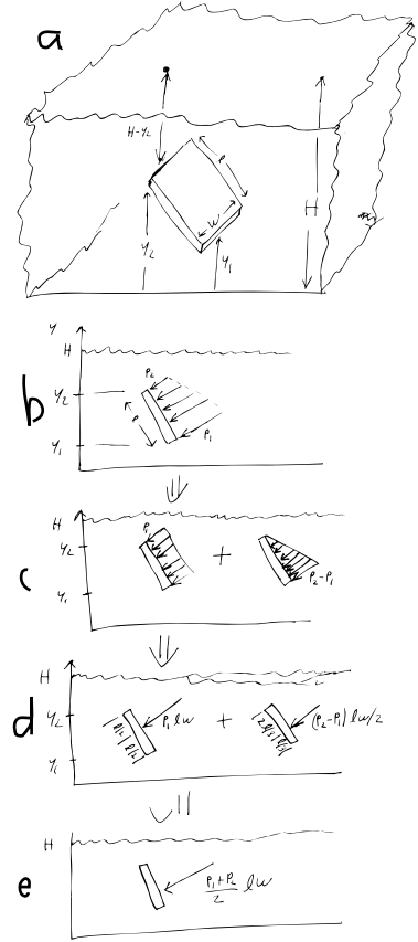
Figure 7.5: The resultant force from a constant depth-increasing pressure on a rectangular plate.
