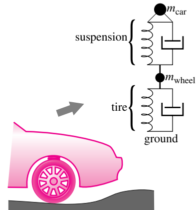
Figure 9.43: The vertical motions of a car and wheel might be considered as coupled motions in 1D.
