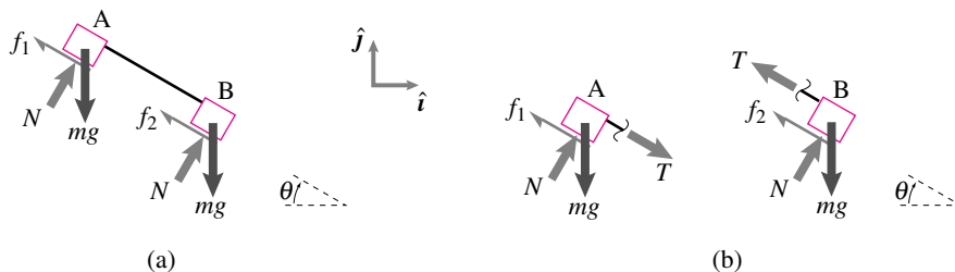
Figure 3.38: Free body diagrams of (a) the two blocks and the rod as a system and (b) the two blocks separately.
