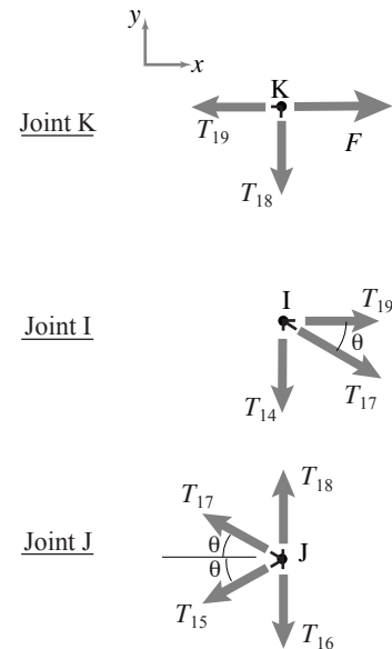
Figure 5.16: Free-body diagrams of joints K, I, and J. From the given geometry, \theta = \tan^{-1}(KJ/IK) = 26.56^\circ .
