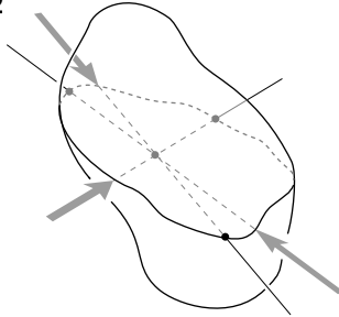
Figure 4.23: If exactly 3 forces act on a body the lines of action of the forces intersect at a single point and are coplanar. The point of intersection does not have to lie within the body. A special case is when that point is at infinity and the three forces are parallel.
