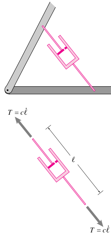
Figure 9.29: A dashpot. A dashpot is shown here connecting two parts of a mechanism. The tension in the dashpot is proportional to the rate at which it lengthens.
