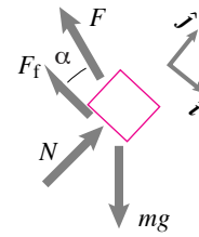
Figure 4.45: Free body diagram of the block. The friction force \vec{F}_f may be known or unknown depending on whether the block is sliding or not. Under downhill sliding, F_f = \mu N , whereas for no sliding |F_f| \leq \mu N .
