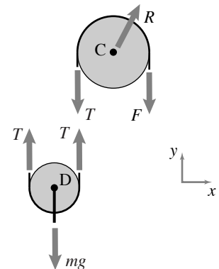
Figure 6.45: Free-body diagram of the two pulleys. We use C and D to designate both the pulleys and their respective centers.
