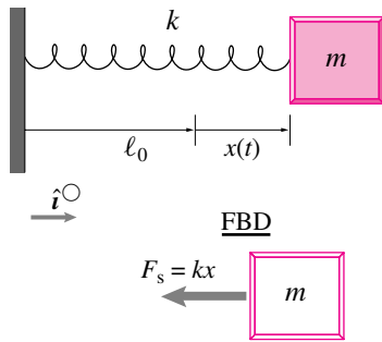
Figure 9.20: A spring mass system. For simplicity, because we are only doing a 1D analysis, not shown on the FBD are forces that have no component in the relevant direction such as from gravity or the (assumed massless and frictionless) support wheels. It would be more correct to show those forces, but it would add clutter to the picture.
