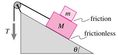
Figure 3.35: Two blocks held in place on an inclined surface
