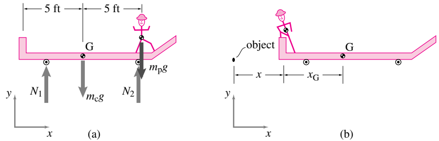
Figure 9.60: (a) Free-body diagram of Mr. P-and-the-cart system. (b) The cart has moved to the right by distance x when Mr. P reaches the other end.
