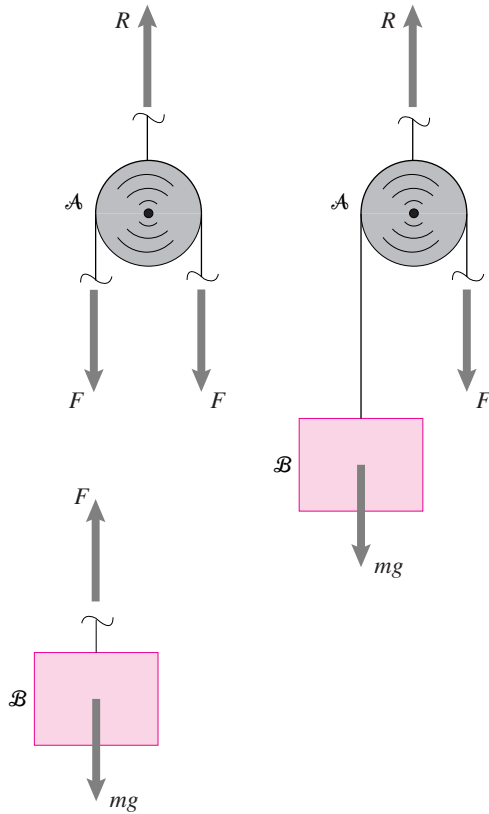
Figure 3.12: The free-body diagrams of the mass, the pulley, and the mass-pulley system. Note that for the purpose of drawing the free-body diagram we need not show that we know that R = 2F . Similarly, we could have chosen to show two different rope tensions on the sides of the pulley and reasoned that they are equal as is done in the text.
