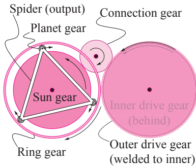
Figure 6.34: A high gain planetary gear system, so named because the ‘planet’ gears go around the ‘sun’ gear. Often planetary gears depend on the sun or the spider or the ring not rotating. In this design all three rotate. A CCW torque is applied to the Inner drive gear which is welded to the outer drive gear. The outer drive gear turns the ring gear CW. The inner drive gear turns the the connection gear CW which turns the sun gear CCW. The three planet gears spin between the inside of the ring gear and the outside of the sun gear. If the inside of the ring gear moves a little faster down than the outside of the sun gear moves up, then the spider turns CW with the center of the planet gears.
