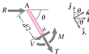
Figure 4.69: Free body diagram of the upper part of the ladder cut at section a-a . Note that \hat{\lambda} = \cos \theta \hat{i} - \sin \theta \hat{j} and \hat{n} = \sin \theta \hat{i} + \cos \theta \hat{j} .
