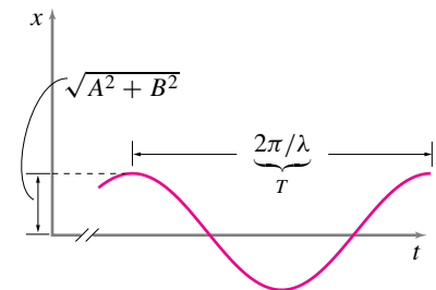
Figure 9.21: Position versus time for an undamped, unforced harmonic oscillator. x is the position of the mass, t is time.
