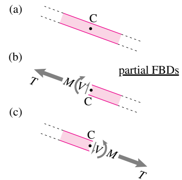
Figure 4.61: a) A piece of a structure, loads not shown; b) a partial free body diagram of the right part of the bar; c) a partial free body diagram of the left part of the bar.
