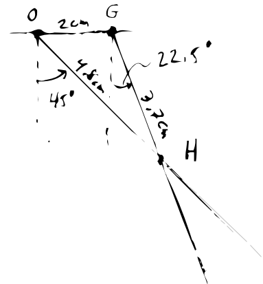
Figure 2.45: Method III: Find point H as the intersection of two known lines.
