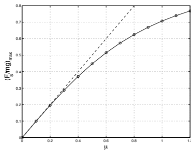
Figure 4.56: The maximum net friction force on the box as a function of the friction coefficient \mu . Note that the relationship is almost linear for most practical values of \mu .
