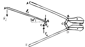
Filename:pfig6-toggle-cutter
