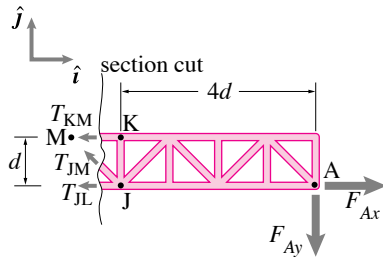
Figure 5.22: Free body diagram of a 'section' of the structure.
