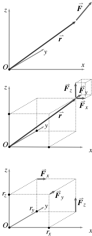
Figure 2.30: The three components of the 3D moment vector are the moments about the three axis. These can be found by sequentially breaking the force into components, sliding each component along its line of action to the coordinate planes, and noting the contribution of each component to moment about each axis. See Fig. 2.23 on page 74 for the 2D version of this construction.
