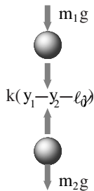
Figure 9.54: Free body diagram of the two masses m_1 and m_2
