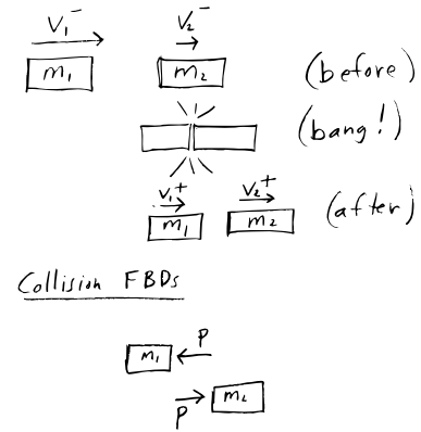
Figure 9.68: Before the collisions the masses have velocities to the right of v_1^- and v_2^- . After the collision the velocities are v_1^+ and v_2^+ . During the collision the impulse \mathbf{P} acts to the right on mass 2 and to the left on mass 1.
