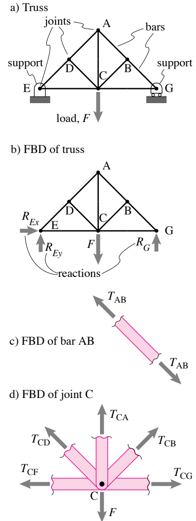
Figure 5.5: a) a truss, b) FBD of truss (It is OK to show R_{Ex} even if it turns out to be zero), c) FBD of a bar, each bar is a two-force body, d) FBD of joint C, a joint is acted on by bar tensions and by applied loads. See Sample 5.1 on page 272 for an analysis of this truss.
