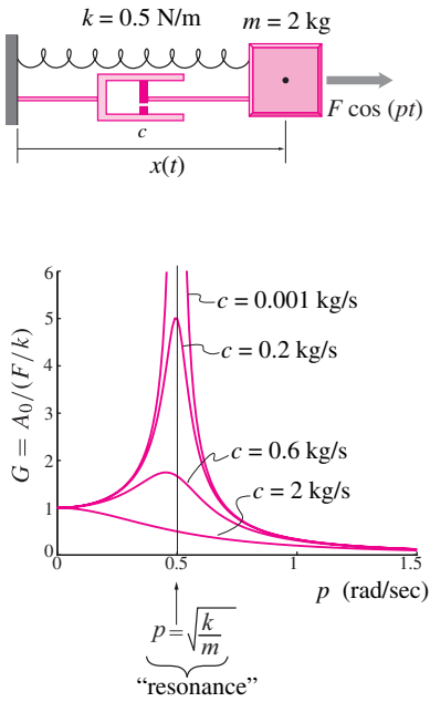
Figure 9.79: Amplitude of oscillation vs forcing frequency for various dampings. Each curve shows the gain G vs the forcing frequency for a fixed damping. Note that when the damping is small ( c \ll 1 ) and the forcing is close to the natural frequency of vibration p \approx \lambda_n there is a 'resonant' peak in the amplitude of the response. The smaller the damping the higher and narrower is this peak. For very high damping the peak is at a slightly lower frequency. The mass-spring-dashpot system shown was used to generate the plots using the formulas from box 9.10 on page 524.
