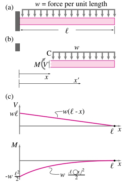
Figure 8.3: a) Cantilever beam, b) free body diagram, c) Shear force diagram, d) Bending moment diagram
