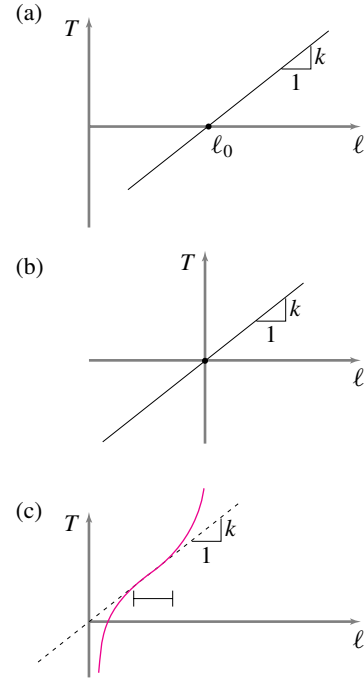
Figure 6.4: a) Tension versus length for an ideal spring, b) for a zero-length spring, and c) for a strip of rubber.
