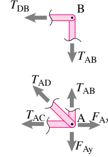
Figure 5.8: Free body diagram of joints B and A.
