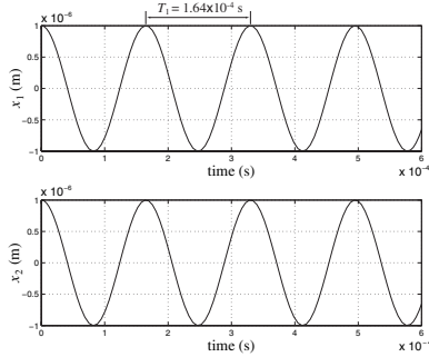
Figure 9.64: Motions of mass A and mass B, x_1(t) and x_2(t) in the first normal mode. Note that both masses move together (in phase) and oscillate with the same frequency, \lambda_n^{(1)} . In this mode, the middle spring, k_2 plays no role as it remains unstretched at all times x_2(t) - x_1(t) = 0 for all t .
