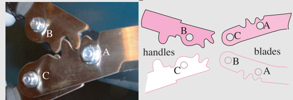
Mechanism details.
