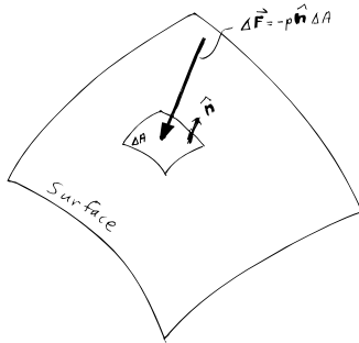
Figure 7.1: A bit of area \Delta A on a surface on which pressure p acts. The outward (into the water) normal of the surface is \hat{n} so the force is \Delta \vec{F} = -p \hat{n} \Delta A .
