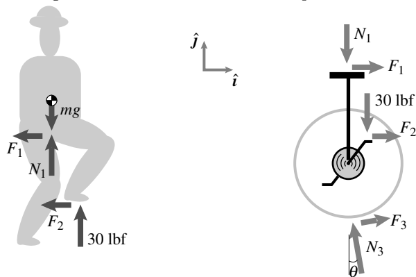
Figure 3.42: Free-body diagram of the cyclist and the cycle.
