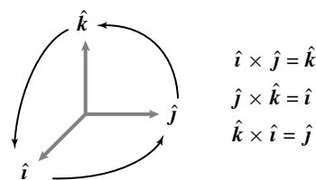
Figure 2.28: Mnemonic device to remember the cross product of the standard base unit vectors.
