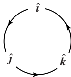
Figure 2.39: The cross product of any two basis vectors is positive in the direction of the arrow and negative if carried out backwards, e.g. \hat{i} \times \hat{j} = \hat{k} but \hat{j} \times \hat{i} = -\hat{k} .
