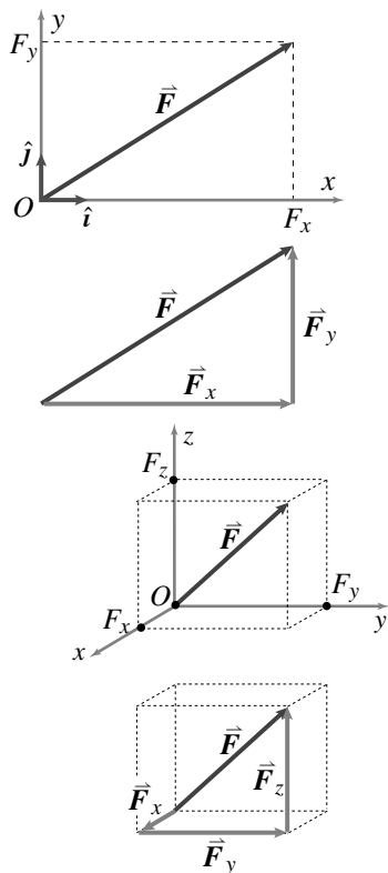
Figure 2.9: A vector can be broken into a sum of vectors, each parallel to the axis of a coordinate system. Each of these is a component multiplied by a unit vector along the coordinate axis, e.g. , \vec{F}_x = F_x \hat{i} .
