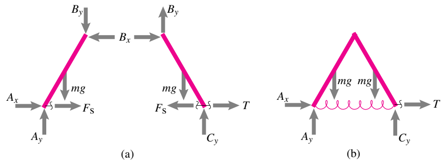
Figure 3.20: Free body diagrams of (a) the individual bars and (b) the structure as a whole.
