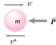
Figure 9.72: Free body diagram of the ball during collision with collisional impulse \vec{P} acting on it.
