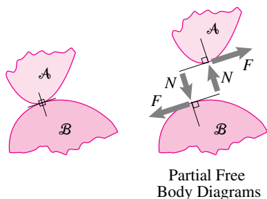
Figure 3.25: Two bodies in contact. The forces between them satisfy the law of action and re-action. It is often convenient to decompose the force of interaction into a part F tangent to the surface of interaction and a part N perpendicular to the surface of interaction.
