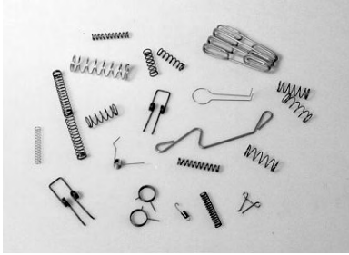
Figure 6.1: Some commercially available springs (Viking Products).
