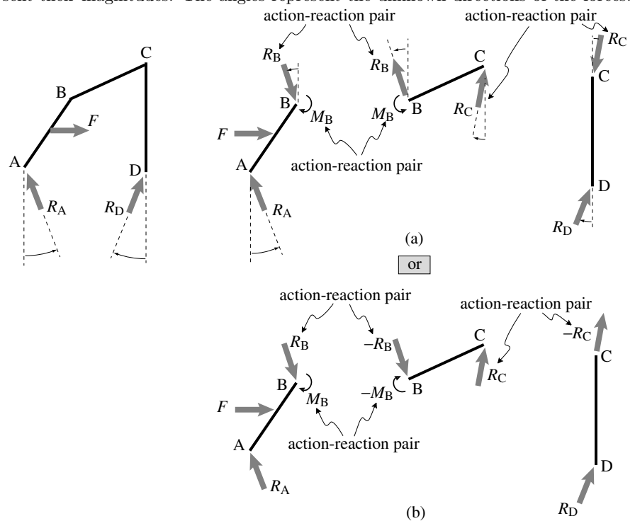
Figure 3.23: Style 2: Free body diagrams of the structure and the individual bars. The forces shown in (a) and (b) are the same.
