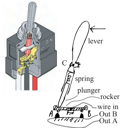
Figure 6.29: Cutaway drawing of a toggle switch and a simplified schematic of the idea. The lever, spring and plunger rotate about C. The spring is prestressed so that the plunger presses hard against the rocker. The plunger slides on the rocker (input line) which is pressed against contact at outputs A or B. The relevant idea here is that the force of the plunger on the rocker can be much bigger than the input force on the lever (cutaway from NKK Switches online catalogue).
