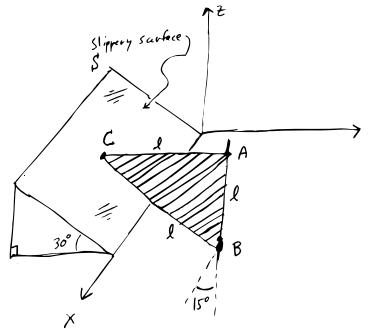
Filename:pfigure-restingtriangle
