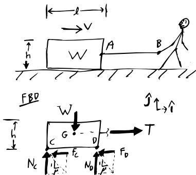
Figure 4.42: Dragging a block, taking account (in a simple way) the distribution of contact forces from the ground. Assume slip to the right is occurring.
