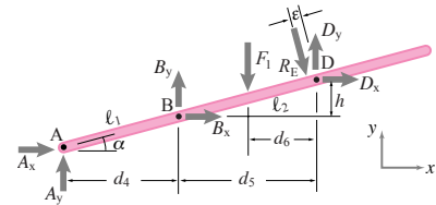
Figure 5.58: Free-body diagram of bar ABD. Note that d_4 = \ell_1 \cos \alpha , d_5 = \ell_2 \cos \alpha , d_6 = d_5/2 = (\ell_2/2) \cos \alpha , and h = \ell_2 \sin \alpha .
