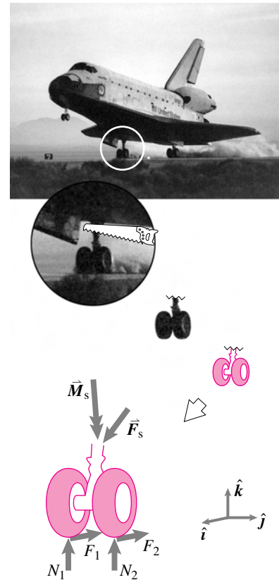
Figure 3.3: The process of drawing a FBD is illustrated by the sequence shown.
