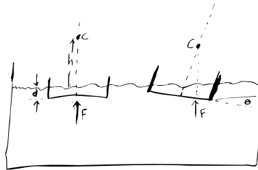
Ship stability.
