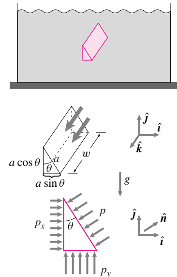
Figure 7.2: A small prism of water is isolated from some water in equilibrium. The free body diagram does not show the forces in the z direction. Force balance applied to this free body diagram shows that p_x = p_y = p , pressure is the same in all directions.
