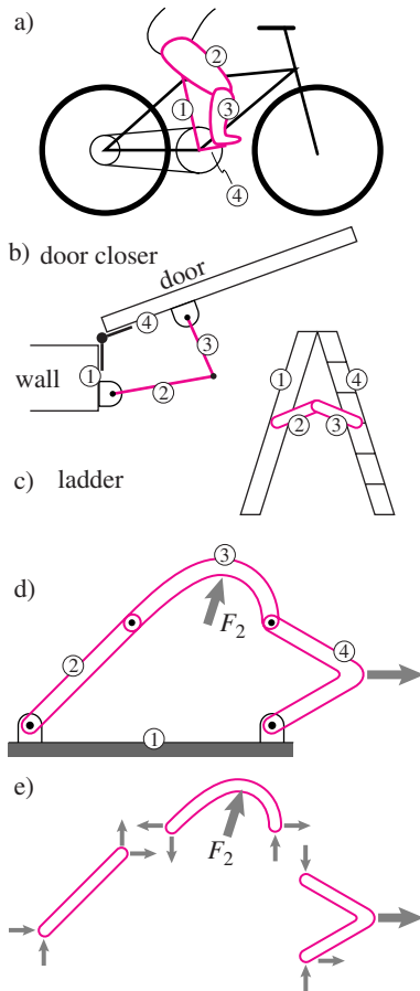
Figure 6.52: Four bar linkages. a) A bicycle, thigh, calf, and crank, b) a door closer, c) a folding ladder, d) a generic mechanism, e) free body diagrams of the parts of a generic mechanism.
