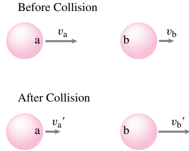
Figure 9.69: The rate of approach of two about-to-collide points is v_a - v_b . The rate of separation after collision is v_b' - v_a' . The simplest collision law says v_b' - v_a' = e(v_a - v_b) , where e is the coefficient of restitution.
