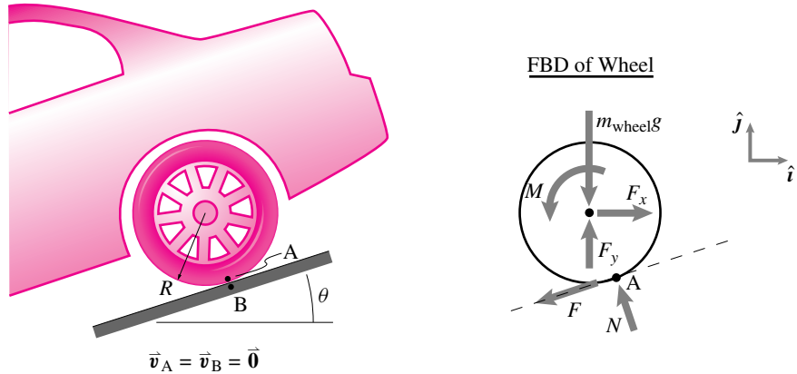
Figure 3.30: Pure rolling of a round wheel on a flat slope in two dimensions.
