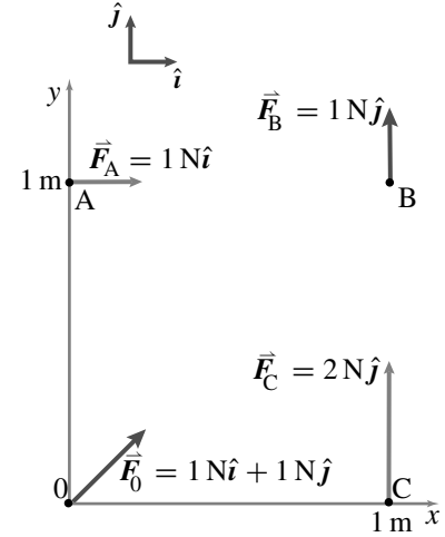
Figure 2.53: The force system \vec{F}_A, \vec{F}_C is equivalent to the force system \vec{F}_0, \vec{F}_B .
