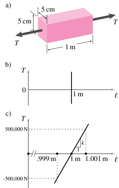
Figure 6.10: a) a steel rod in tension, b) tension versus length curve, c) zoom in on the tension versus length curve.
