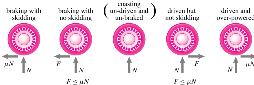
Figure 3.32: Partial free body diagrams of wheel in a braking or accelerating car that is pointed and moving to the right. The force of the ground on the tire is shown. But, for simplicity, the forces of the axle, gravity, and brakes on the wheel are not shown (that's why its a partial FBD). An ideal point-contact wheel is assumed. There is no 'rolling resistance' here.
