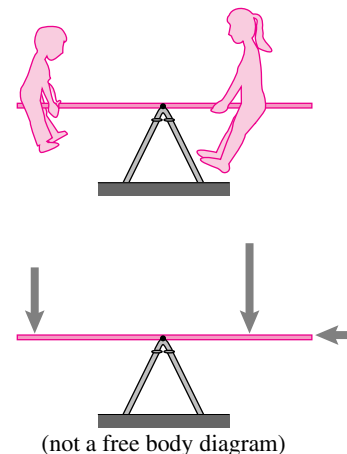
Figure 2.21: On a balanced teeter totter the bigger person gets the short end of the stick. A sideways force directed towards the hinge has no effect on the balance.
