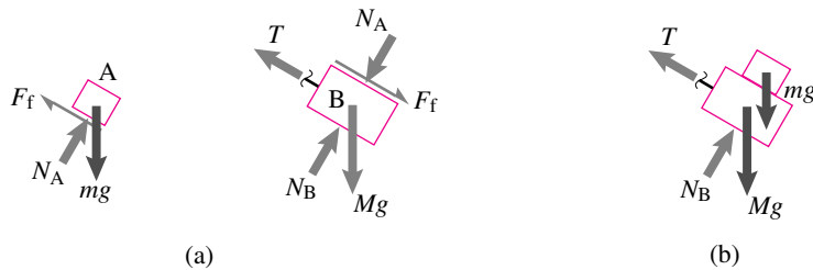
Figure 3.36: Free body diagrams of (a) block A and block B separately and (b) blocks A and B together.
