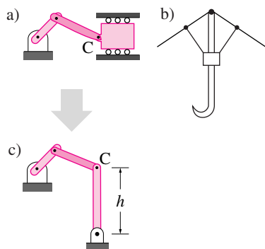
Figure 6.53: a) a slider crank, b) an umbrella has a slider-crank mechanism, c) the equivalent four-bar linkage, at least when h \rightarrow \infty .
