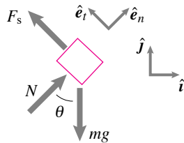
Figure 4.13: Free-body diagram of the mass and the geometry of force vectors.
