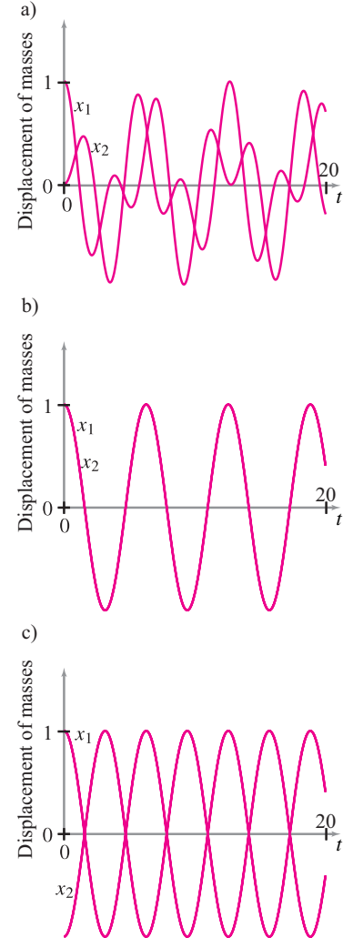
Figure 9.49: Motions of the masses from Fig. 9.48 for three different initial conditions, all released from rest ( v_1 = v_2 = 0 )
