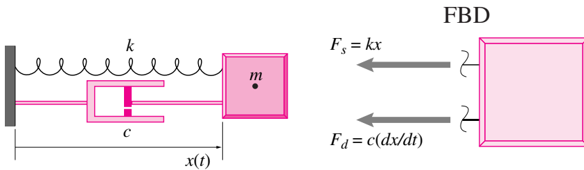
Figure 9.28: A mass spring dashpot system, or damped harmonic oscillator. Also shown is a free body diagram of the mass.
