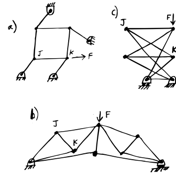
Figure 5.23: Some statically determinate trusses that do not yield easily to the method of sections. No section cut reveals a free body diagram from which you can find T_{JK} . In the truss (c) there are joints only where dots are marked (this mildly unusual truss has no closed triangles). To find T_{JK} in these trusses one has to write the equilibrium equations for many joints and solve these simultaneously.
