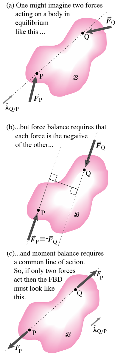
Figure 4.18: (a) Two forces acting on a body \mathcal{B} . (b) force balance implies that the forces are equal in magnitude and opposite in direction ( \vec{F}_P = -\vec{F}_Q ). (c) moment balance implies that the forces are colinear. Body \mathcal{B} is a two-force member; the equilibrium equations imply that the two forces must be equal in magnitude, opposite in direction, and colinear. If the free body diagram shows equal-in-magnitude, opposite-in-direction and colinear forces then the equilibrium equations add no new information.
