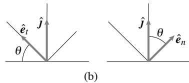
Figure 4.14: (a) Components of mg along t and n directions. (b) The mixed basis dot products: \hat{j} \cdot \hat{e}_t = \sin \theta and \hat{j} \cdot \hat{e}_n = \cos \theta
