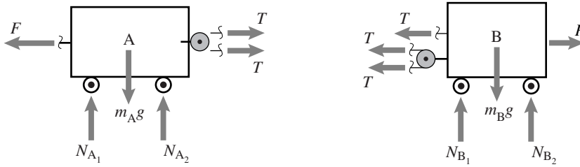
Figure 3.18: Free body diagrams of the two masses.
