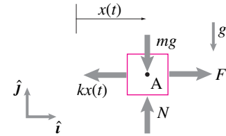
Figure 9.84: Free-body diagram of the mass.
