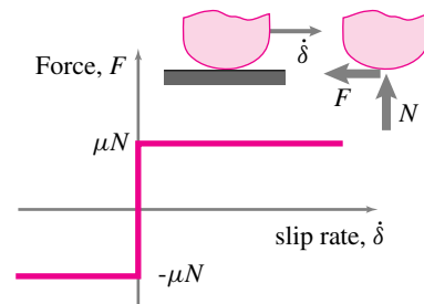
Figure 3.26: Coulomb friction. The relation between friction force F and relative slip rate \dot{\delta} is described by the dark line. Since there is a jump from -\mu N to \mu N in the friction force when the slip rate goes from negative to positive the relation is not a proper mathematical function between F and \dot{\delta} . Instead the relation is a curve in the F, \dot{\delta} plane.
