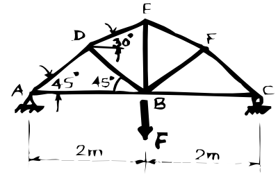
Filename:pfigure4-2-truss2
