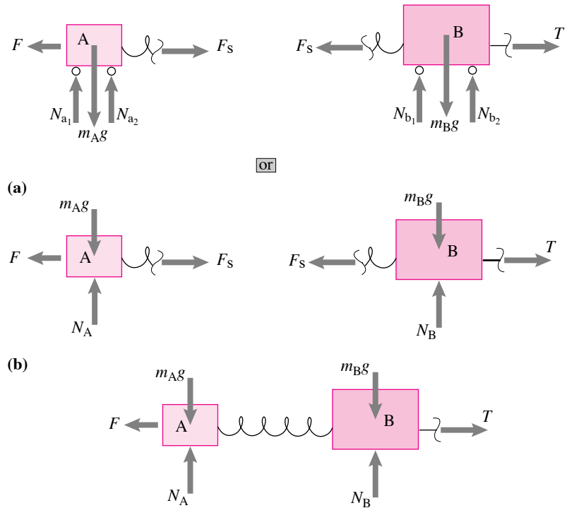
Figure 3.16: Free body diagrams of (a) cart A and cart B separately and (b) cart A and B together
