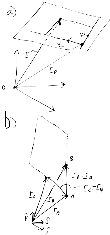
Figure 2.50: a) Parametric equation of a plane. b) the plane through the points A, B, and C
