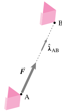
Figure 2.7: The force \vec{F} that points from A to B can be represented as the product of a scalar F and a unit vector \hat{\lambda}_{AB} : \vec{F} = F \hat{\lambda}_{AB} .
