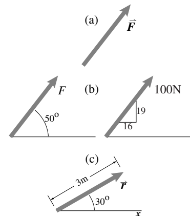
Figure 2.8: Two different ways of drawing a vector (a) Symbolic. The magnitude and direction of the vector is given by the symbol \vec{F} , the drawn arrow has no quantitative information; (b) “Scalar times arrow” shows an arrow with clearly indicated orientation next to the scalar F or the scalar 100N. The vector indicated is the scalar multiplied by a unit vector in the direction drawn; (c) Combined. The symbol \vec{v} is defined (set equal to) a vector with the magnitude and orientation shown.
