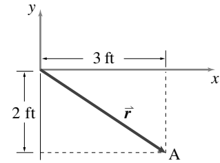
Figure 2.11: A vector \vec{r} = 3\text{ ft}\hat{i} - 2\text{ ft}\hat{j} is drawn by locating its end point which is 3 units away along the x -axis and 2 units away along the negative y -axis.
