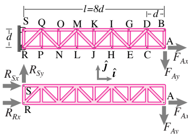
Figure 5.7: A truss with 33 bars, 18 joints and 3 unknown reaction forces. The reactions are sometimes written as, say, R_{S,x} instead of F_{S,x} .
