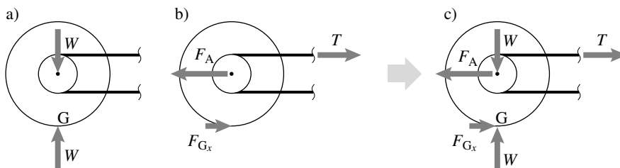
Figure 4.25: A bicycle wheel.
