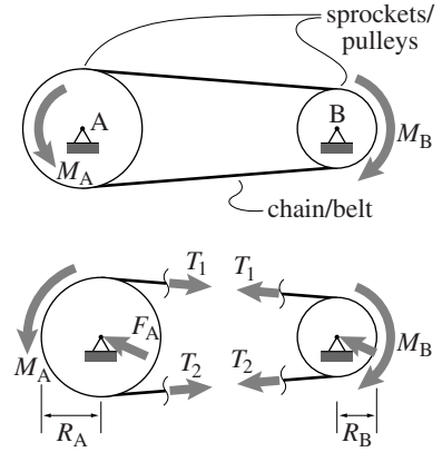
Figure 6.51: a) A chain or pulley drive involving two sprockets or pulleys and one chain or belt, b) free body diagrams of each of the sprockets/pulleys.
