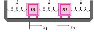
Figure 9.48: A two mass system. We define x_1 and x_2 so that the system is in equilibrium when x_1 = x_2 = 0 .
