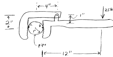
Filename:pfigure-wrench
