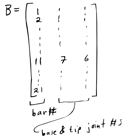
Figure 5.35: The matrix [B] gives the base and tip joint # of each bar.
