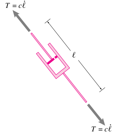
Figure 9.27: A damper or dashpot. The symbol shown represents a device which resists the relative motion of its endpoints. The schematic is supposed to suggest a plunger in a cylinder. For the plunger to move, fluid must leak around the cylinder. This leakage happens for either direction of motion. Thus the damper resists relative motion in either direction; i. e., for \dot{L} > 0 and \dot{L} < 0 .
