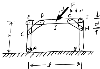
Filename:pfigure-frametable1
