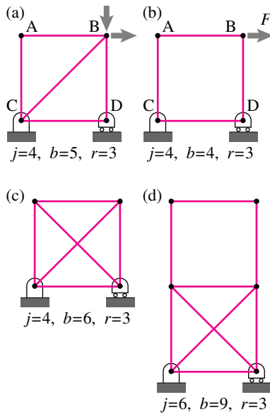
Figure 5.64: a) a statically determinate truss, b) a non-rigid truss, c) a redundant truss, and d) a non-rigid and redundant truss.
