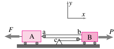
Figure 3.17: Two carts connected by massless pulleys.
