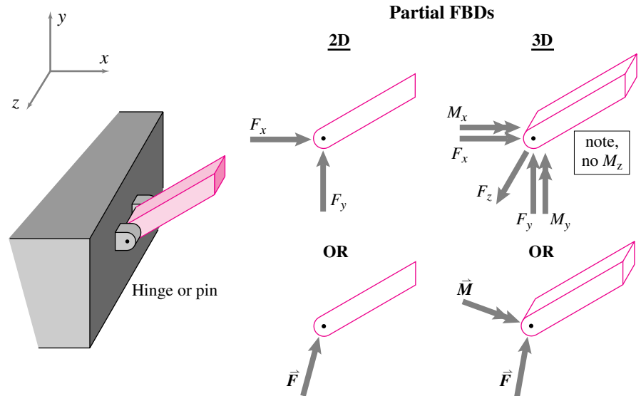
Figure 3.8: A hinge with partial free-body diagrams in 2D and 3-D. A hinge joint is also called a pin joint because it is sometimes built by drilling a hole and inserting a pin.
