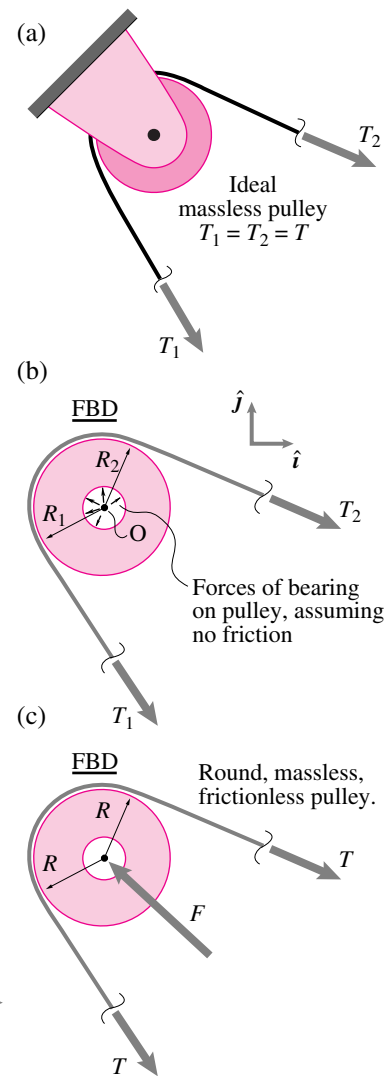
Figure 4.24: (a) An ideal massless pulley, (b) FBD of idealized massless pulley, detailing the frictionless bearing forces and showing forces at the cut strings, (c) final FBD after analysis.
