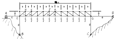
Filename:F02p1p1bridge
