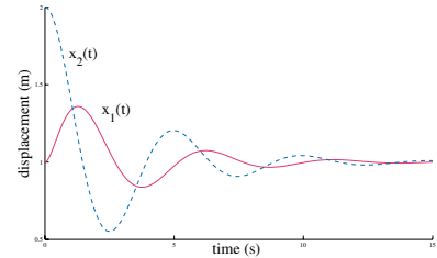
Figure 9.52: Plot of x_1(t) and x_2(t) obtained from the numerical solution of the equations of motion. Note that with x_1(0) = 1 \text{ m} and x_2(0) = 2 \text{ m} , both masses settle down to x_1 = x_2 = 1 \text{ m} after the oscillations die.
