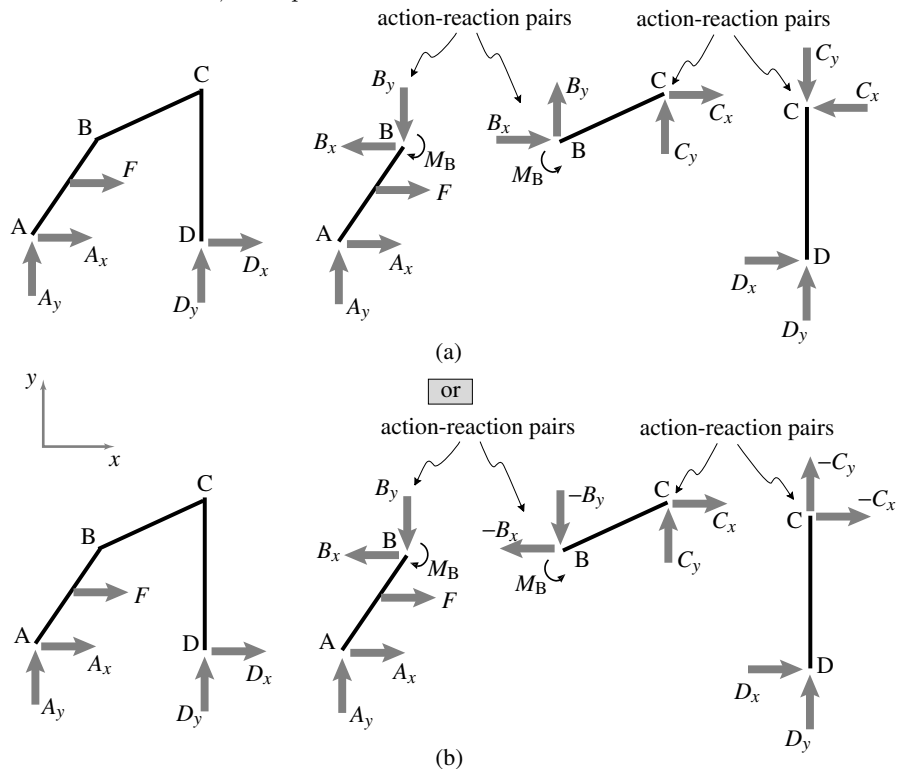
Figure 3.22: Style 1: Free body diagrams of the structure and the individual bars. The forces shown in (a) and (b) are the same.
