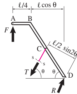
Figure 4.66: Moments of F and T about point D can be evaluated by multiplying the forces with their respective lever arms \ell/4 + \ell\cos\theta and \ell/2\sin 2\theta , respectively.
