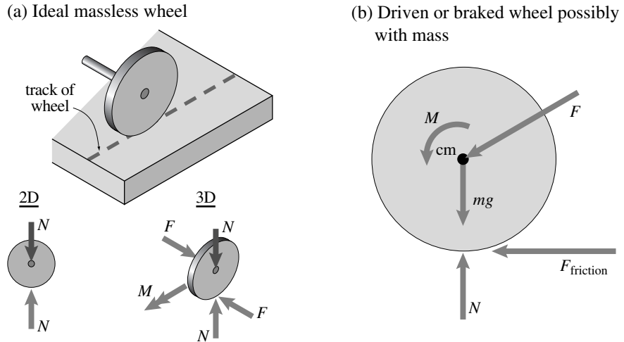
Figure 3.33: An ideal wheel is massless, rigid, undriven, round and rolls on flat rigid ground with no rolling resistance. Free body diagrams of ideal undriven wheels are shown in two and three dimensions. The force F shown in the three-dimensional picture is perpendicular to the path of the wheel. (b) 2D free body diagram of a wheel with mass, possibly driven or braked. If the wheel has mass but is not driven or braked the figure is unchanged but for the moment M being zero.
