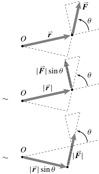
Figure 2.22: The moment of a force |\vec{r}||\vec{F}|\sin\theta is either the product of its distance |\vec{r}| with its perpendicular component |\vec{F}|\sin\theta or of its lever arm (perpendicular distance) |\vec{r}|\sin\theta and the full force |\vec{F}| . The \sim indicates that the lower two forces and positions have the same moment as the force at top.
