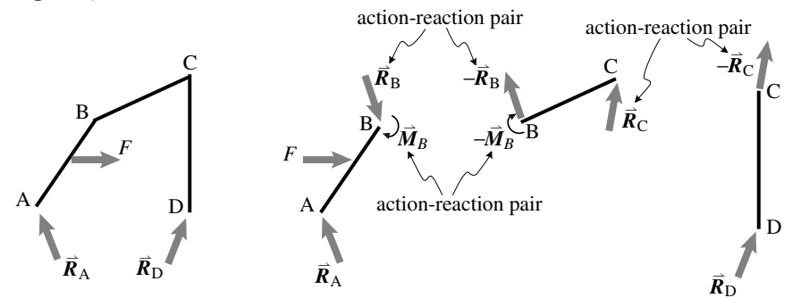
Figure 3.24: Style 3: Free body diagrams of the structure and the individual bars. The label of a force indicates both its magnitude and direction. The arrows are arbitrary and merely indicate that a force or a moment acts on those locations.
