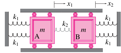
Figure 9.63: The two degree of freedom model of a two-mass MEMS vibratory gyroscope. Here, m = 34.5 \times 10^{-9} kg or 34.5 \mu\text{g} , k_1 = 25 N/m, and k_2 = 3 N/m.
