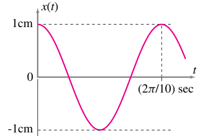
Figure 9.22: The position of a mass as a function of time if k = 50 \text{ N/m} , m = 0.5 \text{ kg} , x(0) = 1 \text{ cm} and v(0) = 0 .
