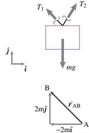
Figure 3.14: Free-body diagram of the block and a diagram of the vector \vec{r}_{AB} .
