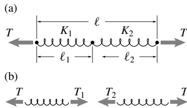
Figure 6.8: Schematic of springs in series.
