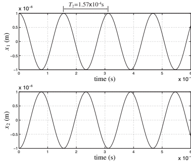
Figure 9.65: Motions of mass A and mass B, x_1(t) and x_2(t) in the second normal mode. In this mode, each mass moves opposite to the other (out of phase) but both oscillate with the same frequency, \lambda_n^{(2)} .
