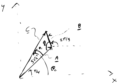
Figure 2.43: Using trig to solve vector triangles
