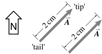
Figure 2.1: Vector \vec{A} is 2 cm long and points Northeast. Two copies of \vec{A} are drawn to show that where the drawing is placed doesn't effect the vector. Its the same vector drawn in two different places.
