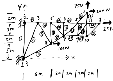
Figure 5.33: A truss with 13 bars (numbered with circles around them), 21 joints, 3 loads and 3 reaction components.
